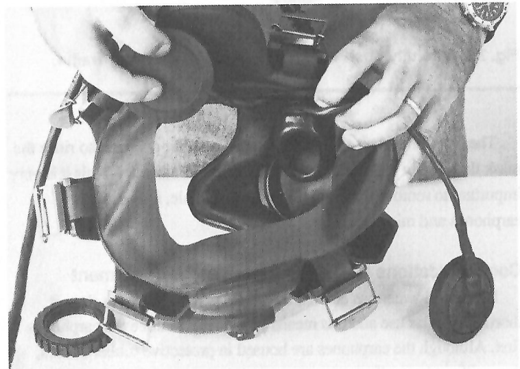
Fig. 7.1 The position of the microphone cup is very important. It must be exactly as it is shown here.
