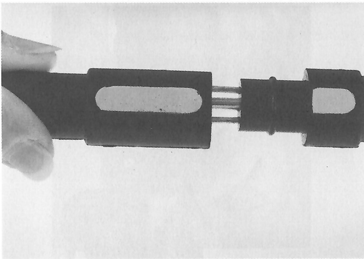
Fig. 5.6 Kintec connectors must be properly aligned when you snap them together. Note the yellow index marks on both the male and female connectors.
