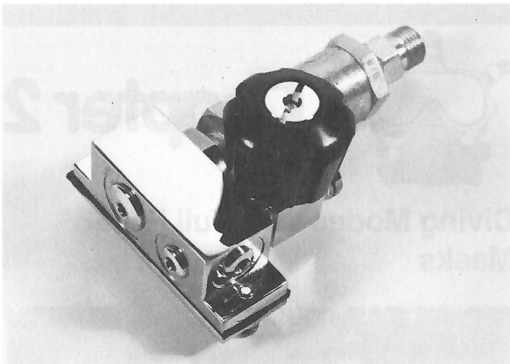
Fig. 2.2 A simple manifold (bail-out) block. (© Diving Systems International. All rights reserved.)
