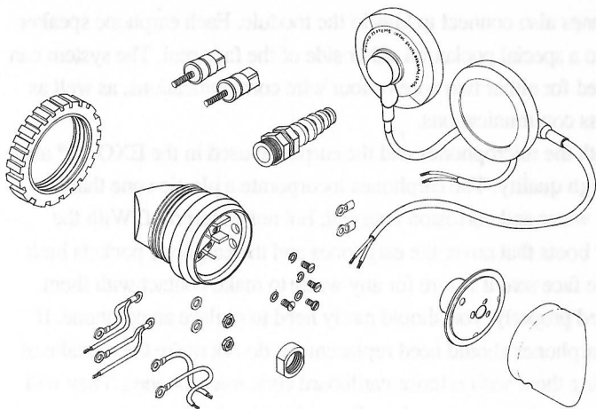
Fig. 4.4 The DSI modular communications system used in the EXO-26® Full Face Mask.
