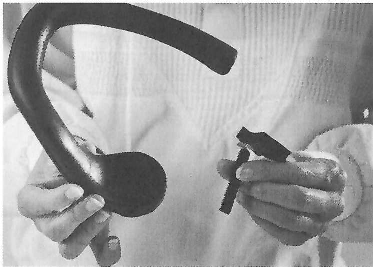
Fig. 4.8 The equalizing device installs on the air delivery tube, which has been removed from the mask to allow you to see where the device is installed.
