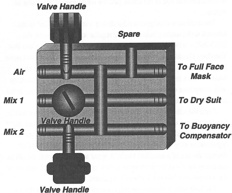
Fig. 2.4 A possible manifold for use with mixed gas scuba.
