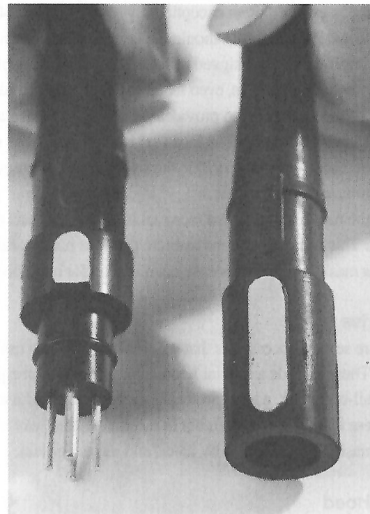
Fig. 4.5 Male and female Kintec four pin waterproof connectors.
