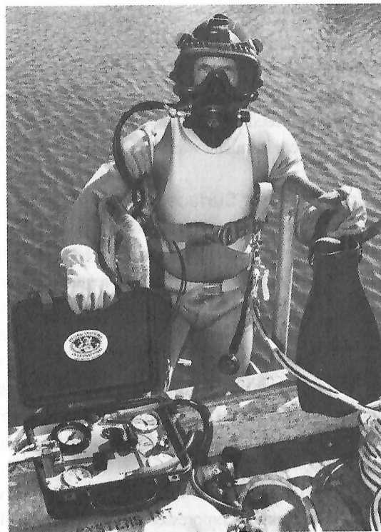
Fig. 6.2 You can put together a complete surface supplied diving system like this for well under $5000.00. The manifold box shown here is the DCS-3®.
