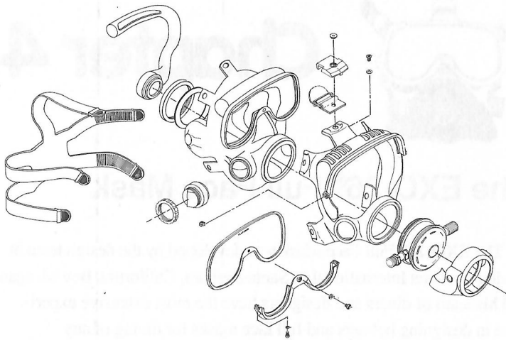
Fig. 4.1 Exploded view of the EXO-26® Full Face Mask. (© 1990 Diving Systems International. All rights reserved.)
