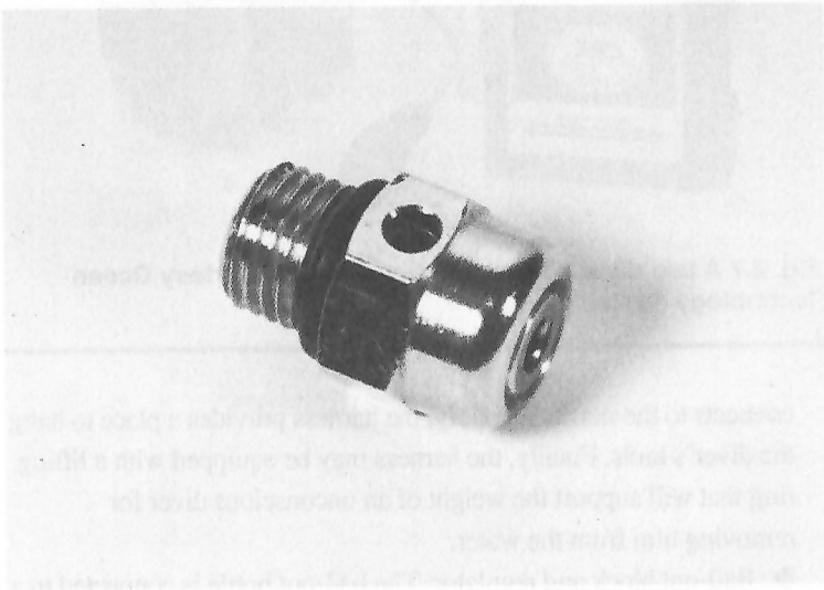
Fig. 2.8 An over-pressure relief valve for use on a first stage regulator. (© Diving Systems International. All rights reserved.)
