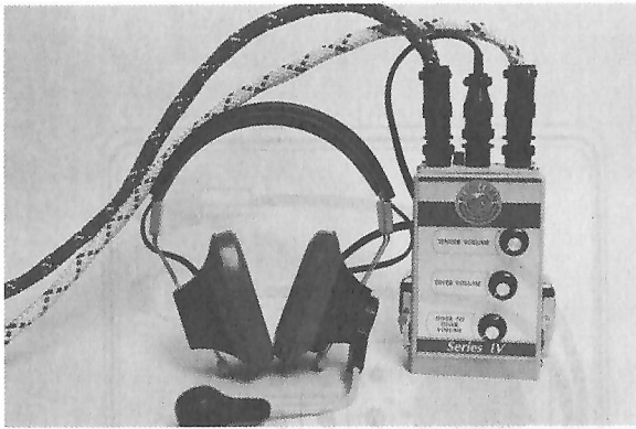
Fig. 6.4 The Buddy Comm Series IV communication system can be used with either tethered scuba or surface supplied air. (Photo courtesy Dive Rescue International.)
