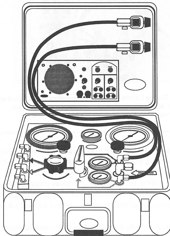
Fig. 6.3 This Dive Control System® can support two divers. (© Diving Systems International. All rights reserved.)
