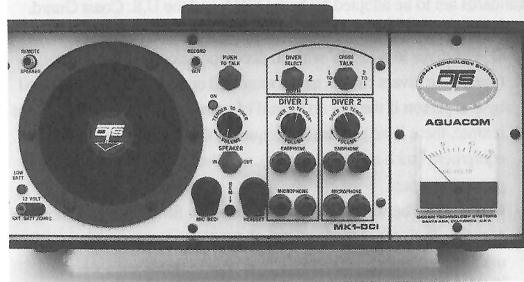
Fig. 6.7 A two diver air diving communications box. (Courtesy of Ocean Technology Systems)
