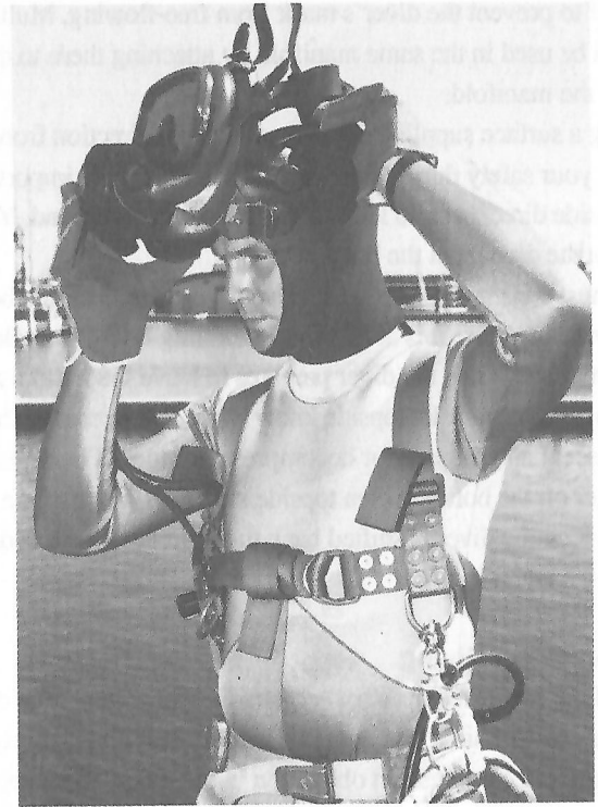
Fig. 6.13 A stainless steel snap hook is used to attach the umbilical to the diver's harness, as can be seen here below the diver's left arm.
