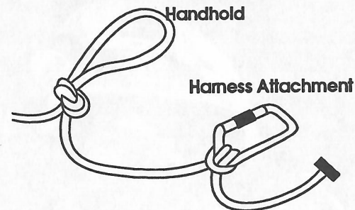
Fig. 5.12 This is one possible comm rope hookup for tethered scuba diving.
