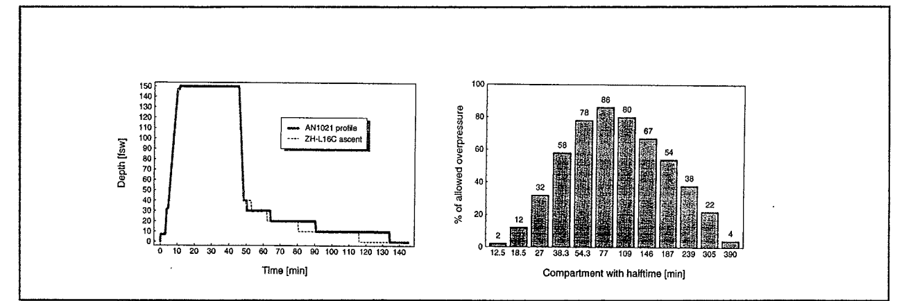
Figure 4. US NEDU wet chamber dive 150 fsw/35.3 min. Left, heavy line shows dive AN1021 (Weathersby et al, 1992) as performed; dashed line is response of model ZH-L16C (Bühlmann, 1993) to same profile, showing a shorter decompression. Outcome, DCS/dives = 1/10 = 10%; 95% confidence limits for 1 of 10 = 0.25–44.5%. DCS risk calculated according to NMRI risk estimation model EE2-2b (Parker et al, 1992): AN1021 profile P_{DCS} = 7.62%; ZH-L16C ascent P_{DCS} = 8.60%. Right, compartment overpressure for AN1021 profile at final surfacing, in % of "allowed" overpressure according to ZH-L16C.
