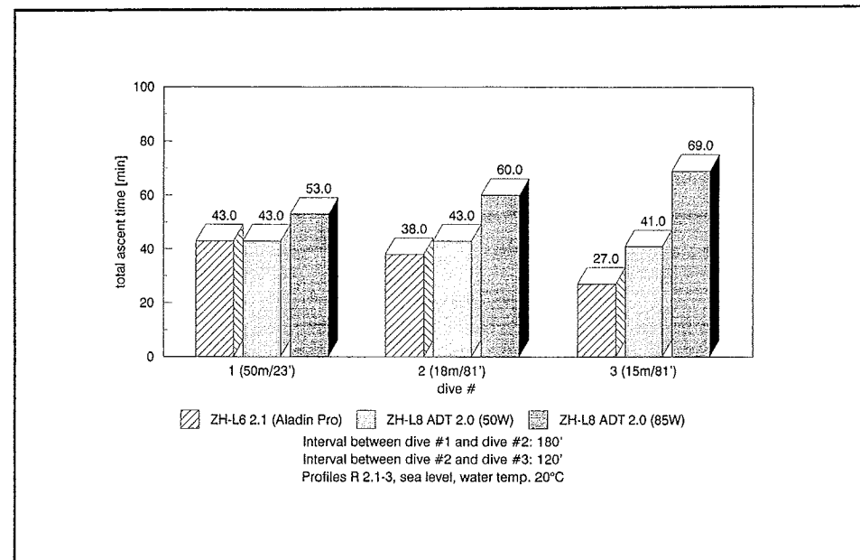
Figure 4. Three dives in warm water. Effect of a high work load on the total ascent time (see also Table 2).
