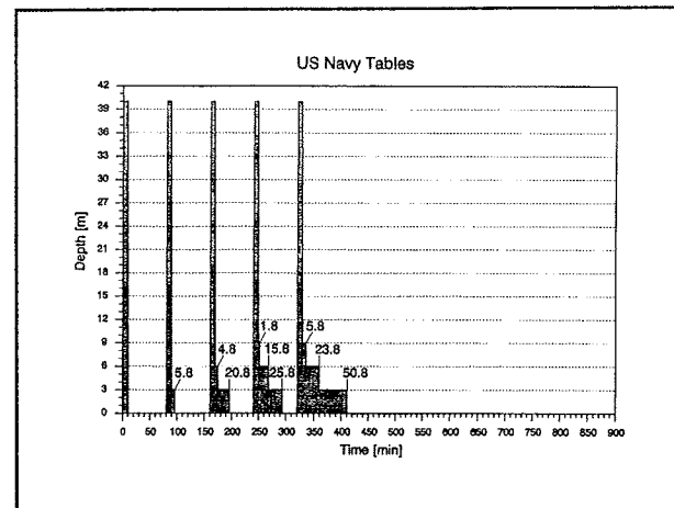
Figure 1. Response of US Navy air decompression tables to yo-yo dives, with descents in one minute to 40 m, holds at 40 m for 7.5 minutes, and ascents at 18 m/min. Descents repeated every 80 minutes.
