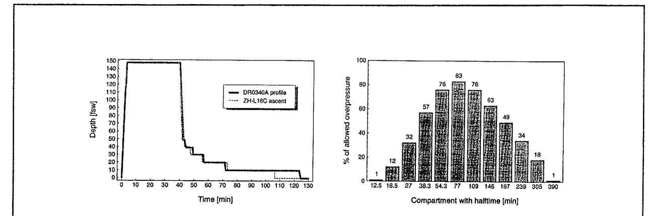
Figure 5. DCIEM dry chamber dive 148 fsw/36.7 min. Left, heavy line is DCIEM dry chamber dive DR0340A (Weathersby et al, 1992), dashed line is response of model ZH-L16C (Bühlmann, 1993) to this profile. DCS/dives = 3/11 = 27.27%; 95% confidence limits 6.02–60.97%. Calculated risk according to NMRI risk estimation model EE2 (2b) (Parker et al, 1992): DR0340A profile P_{DCS} = 7.55%; ZH-L16C ascent P_{DCS} = 8.39%. Right, compartment overpressures for this profile at final surfacing, in % of "allowed" overpressure according to ZH-L16C "Computer" model (Bühlmann, 1993).
