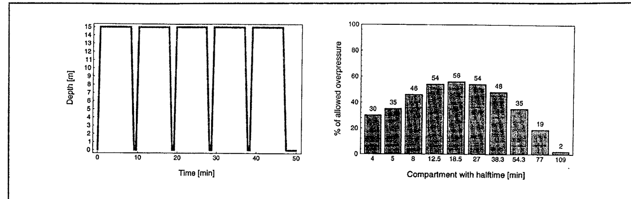
Figure 9. Fish-farming yo-yo profile resulting in DCS (left). Musculoskeletal DCS successfully treated with US Navy Table 6 (Douglas and Milne, 1991). Right, the comparatively low supersaturation by ZH-L16C model (Bühlmann, 1993).
