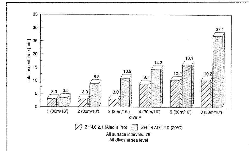
Figure 2. Comparison of ZH-L6 and ZH-L8 ADT: Extensive repetitive diving. Six dives to 30 msw, each with 16 min at 30 msw including 1 min descent time, with 75 min surface intervals. Comparison shows the total ascent time using the Aladin Pro (ZH-L6 2.1) and the Self-Adapting-Dive-Computer (ZH-L8 ADT).
